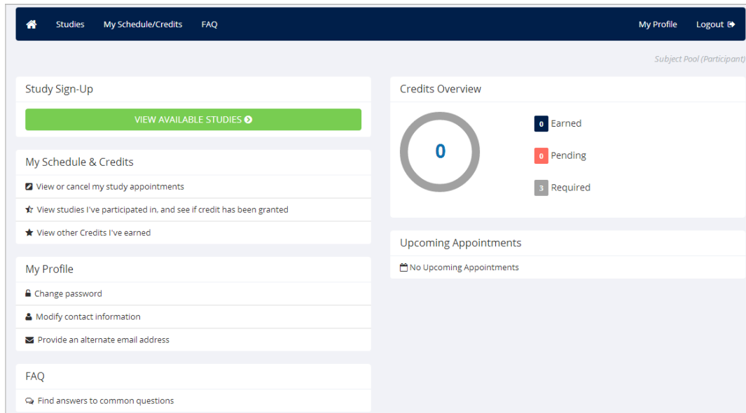
Figure 2 - Main Menu
